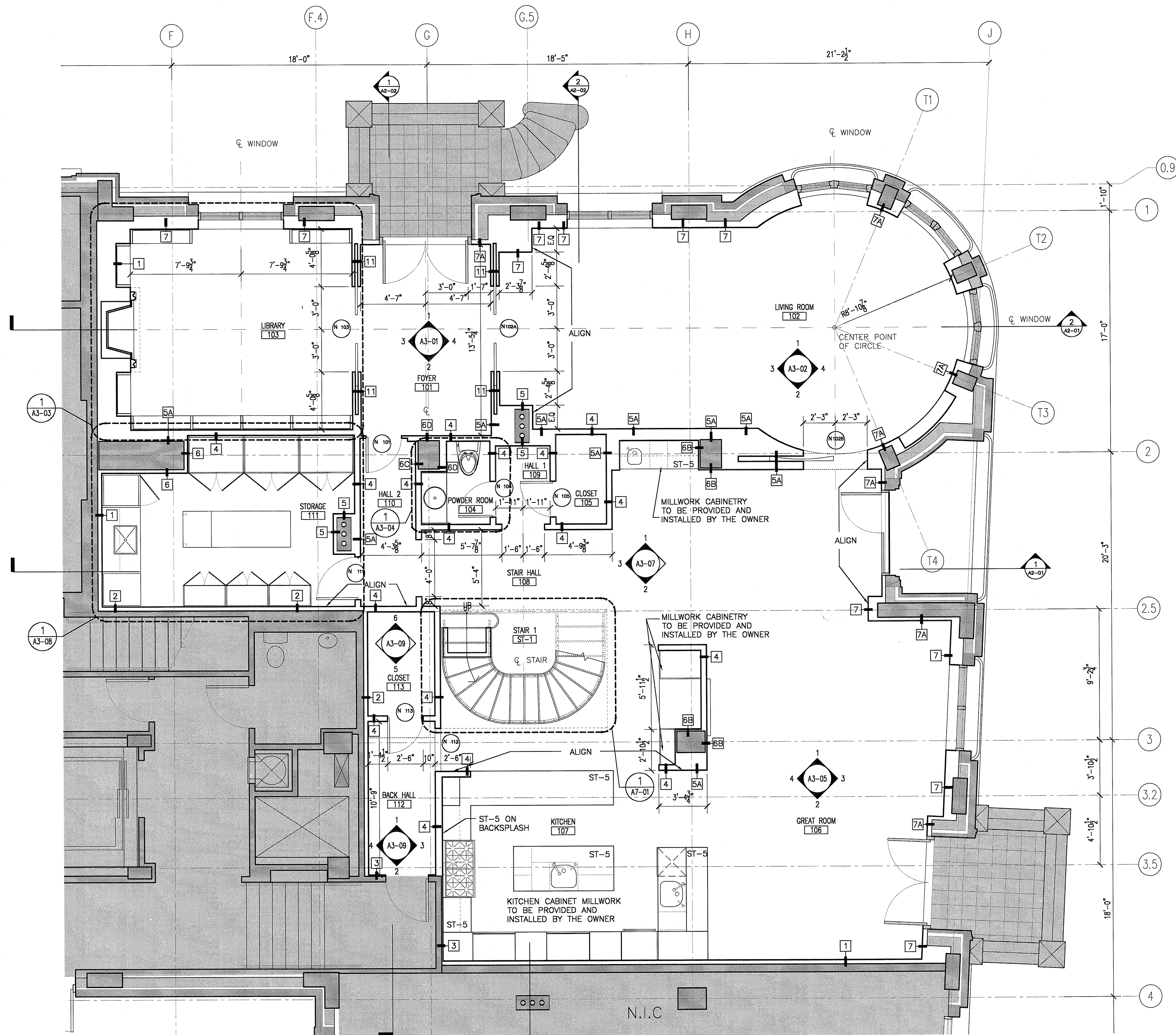
1 GROUND FLOOR PLAN 1/4" = 1'-0"
