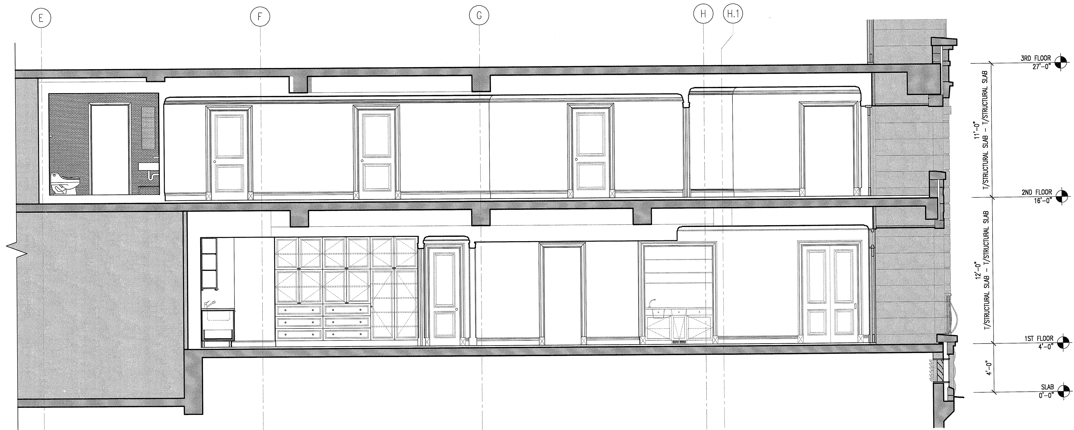
1 SECTION EAST/WEST 1/4"=1'-0"
