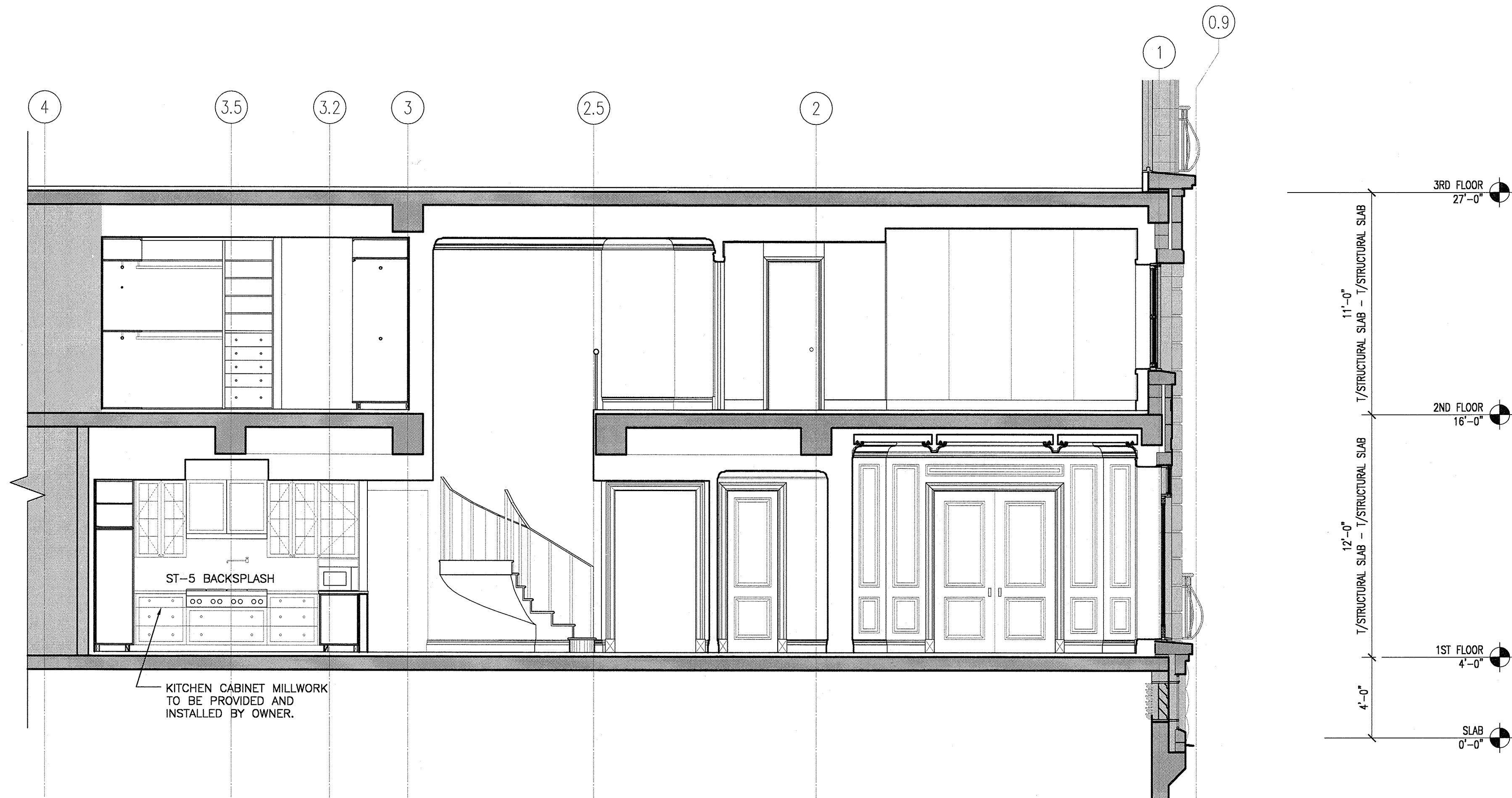
2 SECTION NORTH/SOUTH 1/4"=1'-0"
