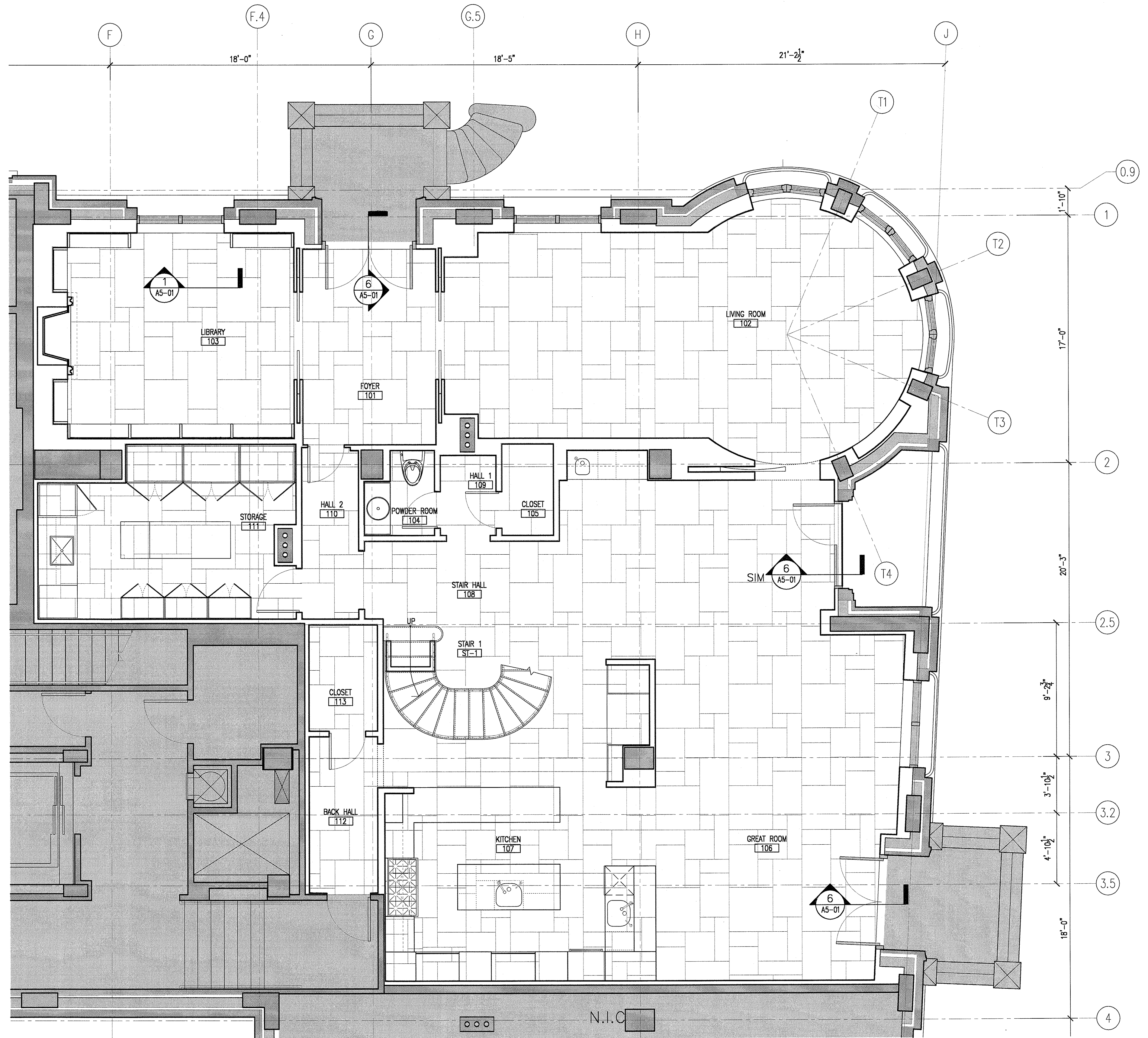
1 GROUND FLOOR FLOOR FINISH PLAN 1/4" = 1'-0"
