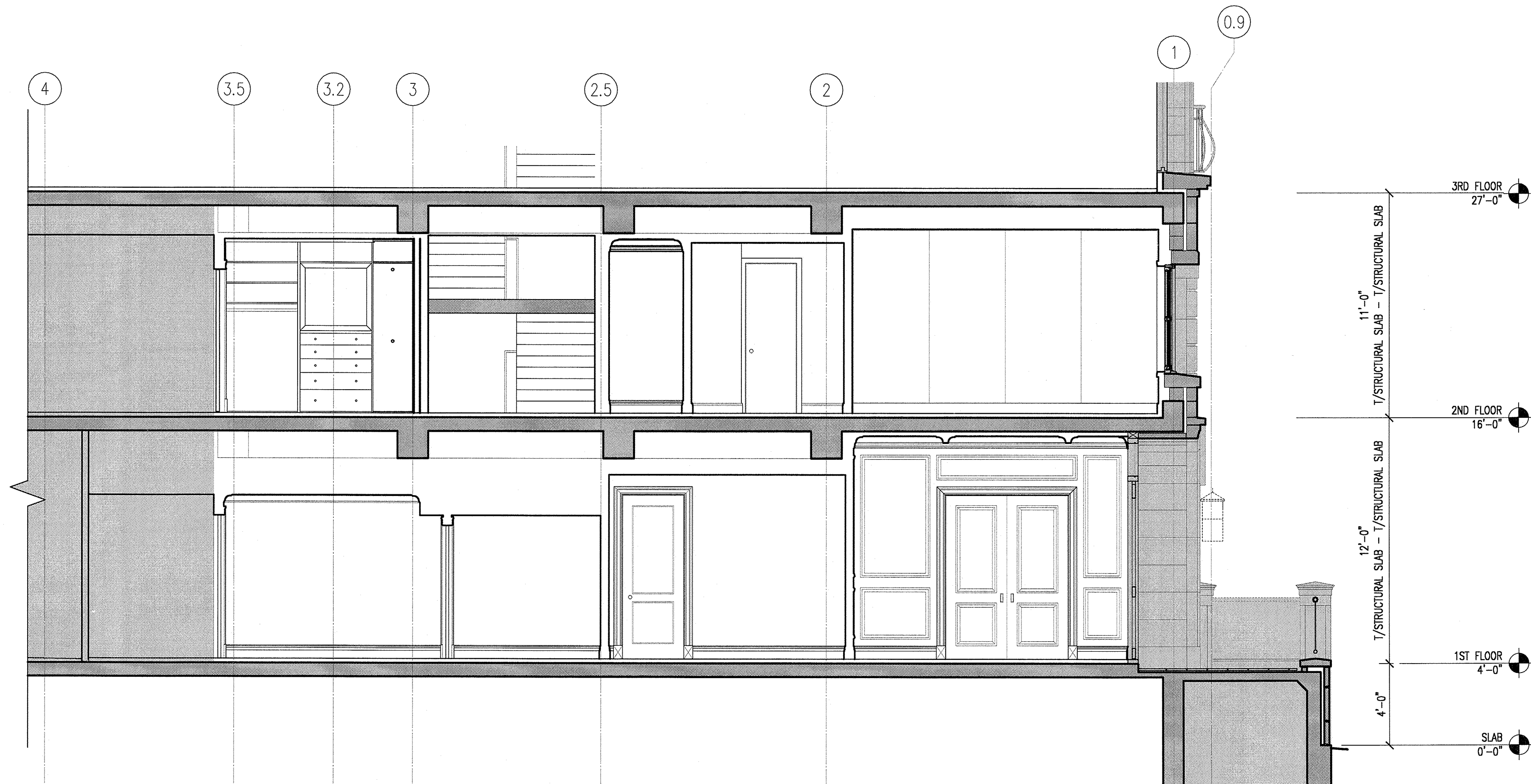
1 SECTION NORTH/SOUTH 1/4"=1'-0"
