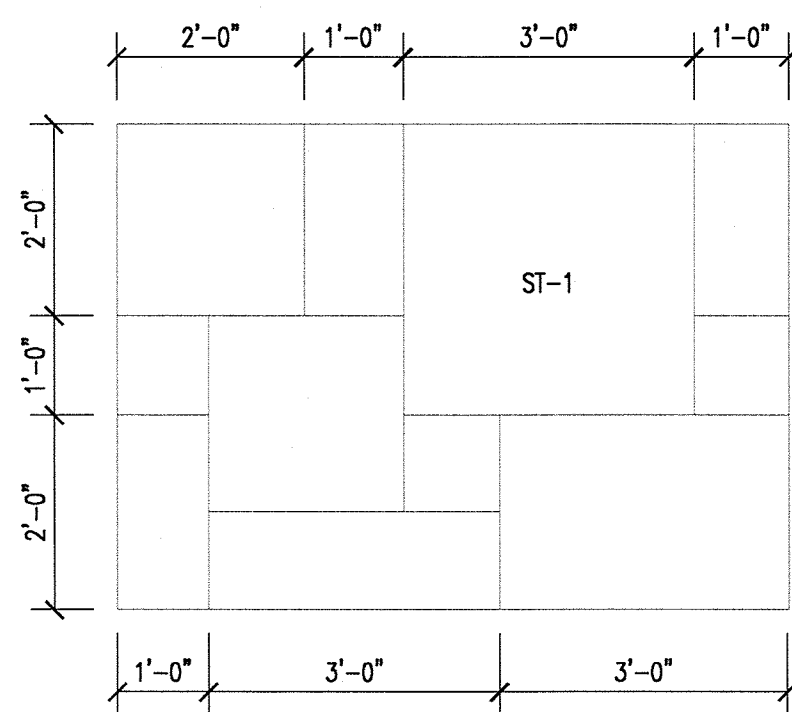
2 RANDOM COURSED RANDOM SIZED STONE PATTERN 1/2" = 1'-0"
