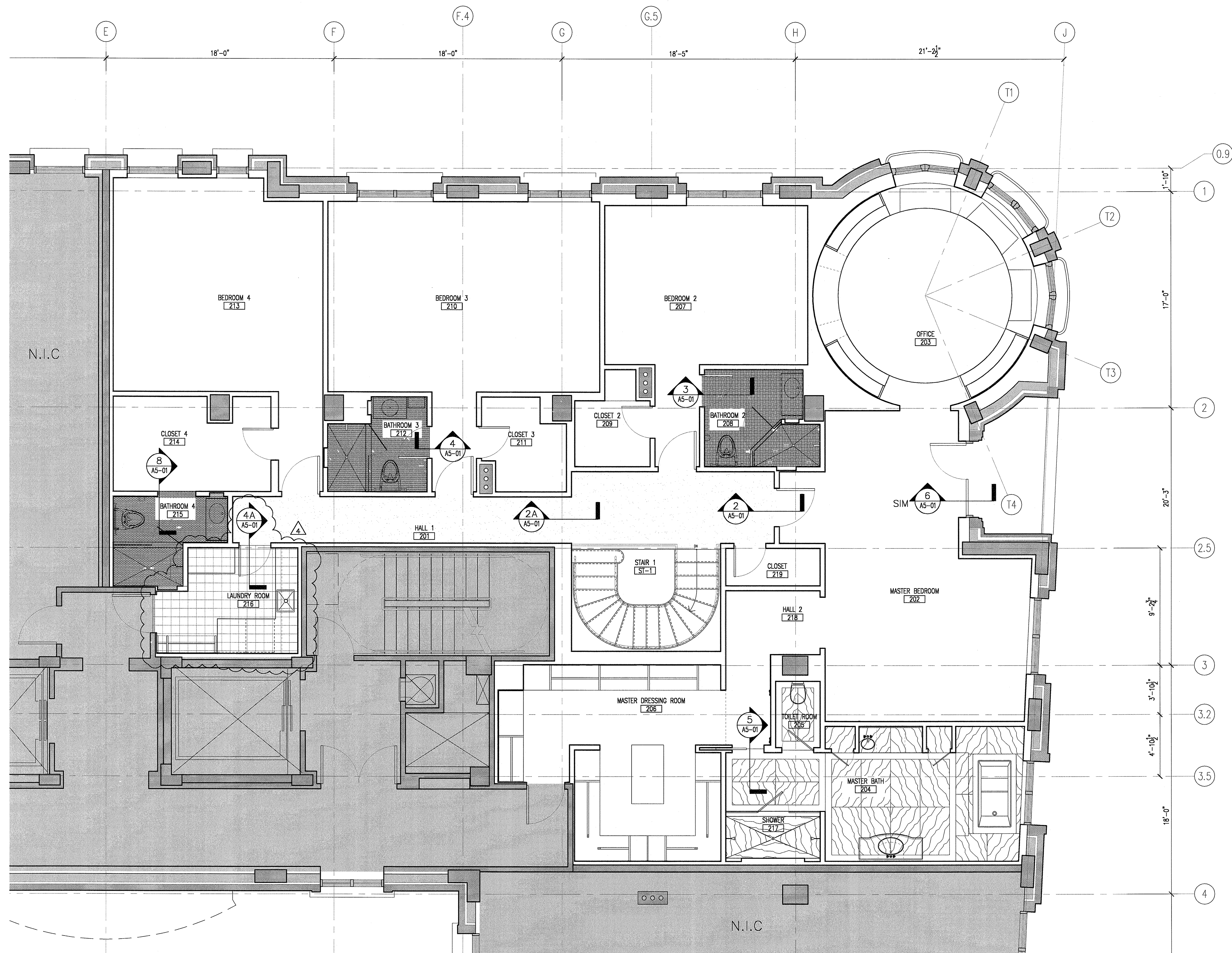
1 SECOND FLOOR FLOOR FINISH PLAN 1/4" = 1'-0"
